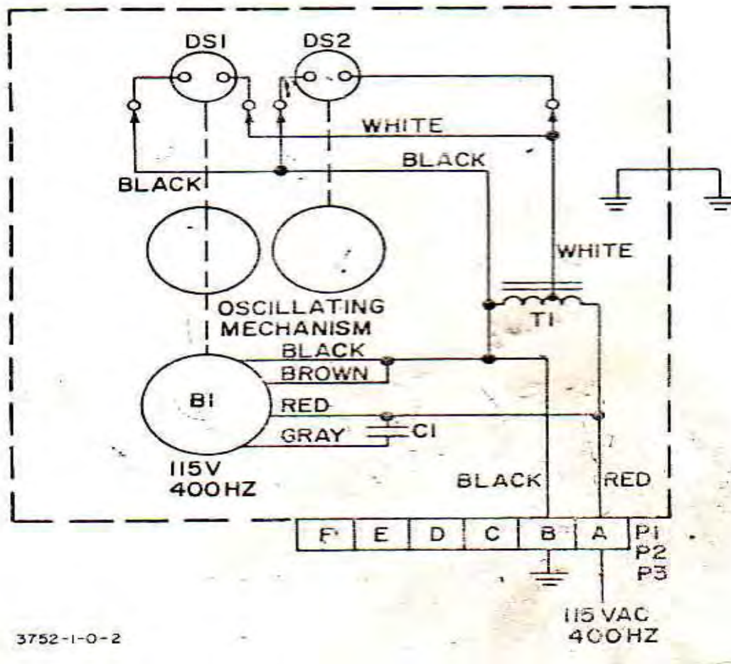
Gambar 7.15 (Wiring Tandem Oscillating Light)
