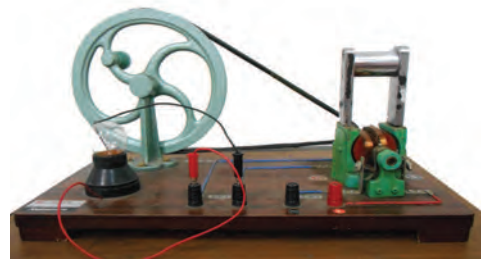
Gambar 6.33 Dinamo AC/DC
