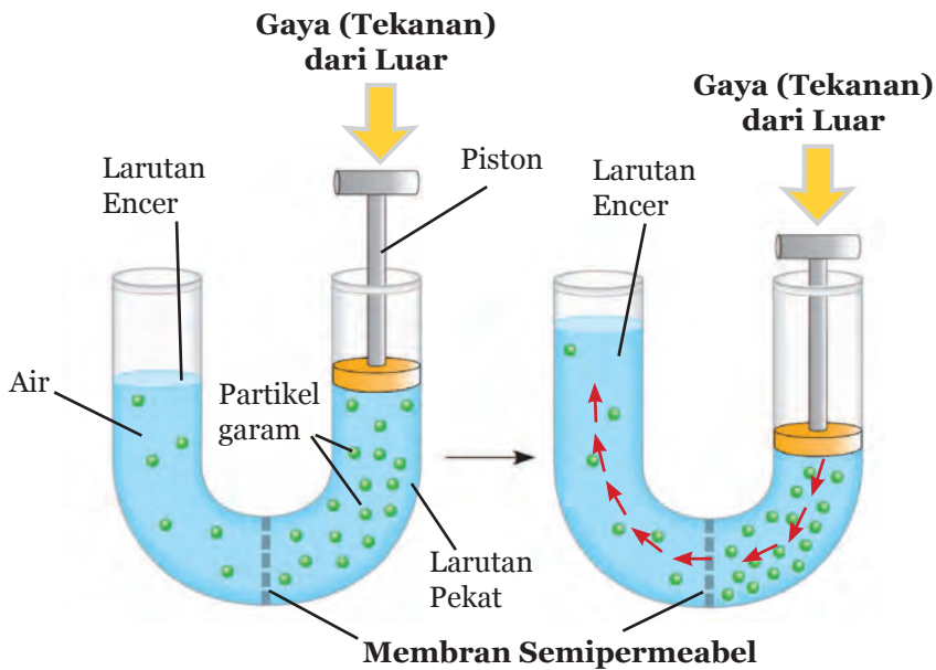
Gambar 9.18 Skema Set Percobaan Osmosis Balik
