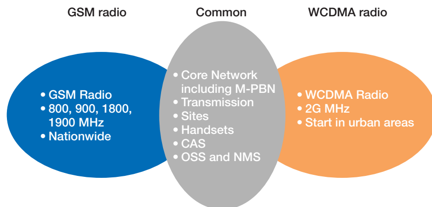
Figure 2: The Ericsson Seamless Network
