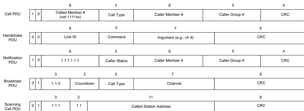
Figure 2: 3G-ALE Protocol Data Units
